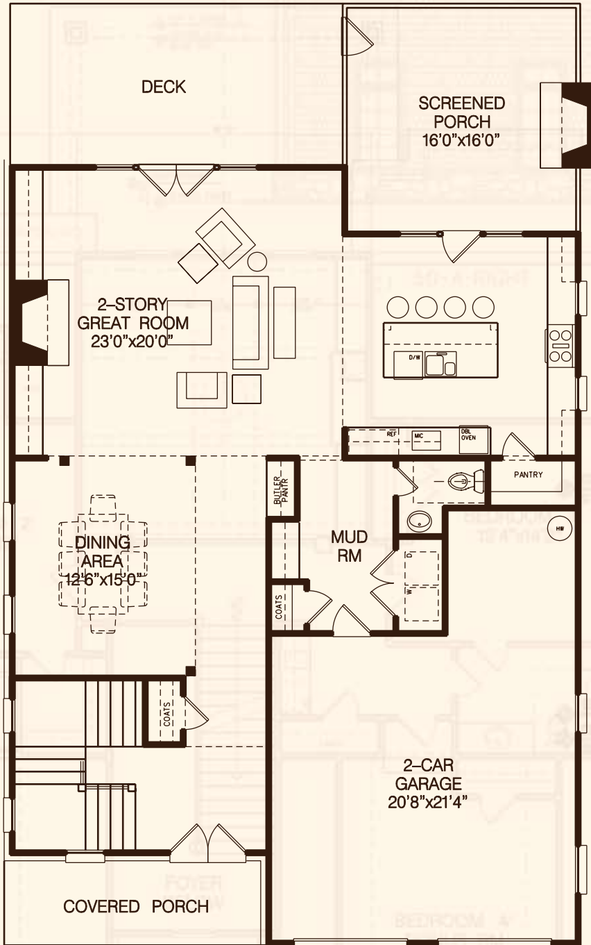
MAIN LEVEL
